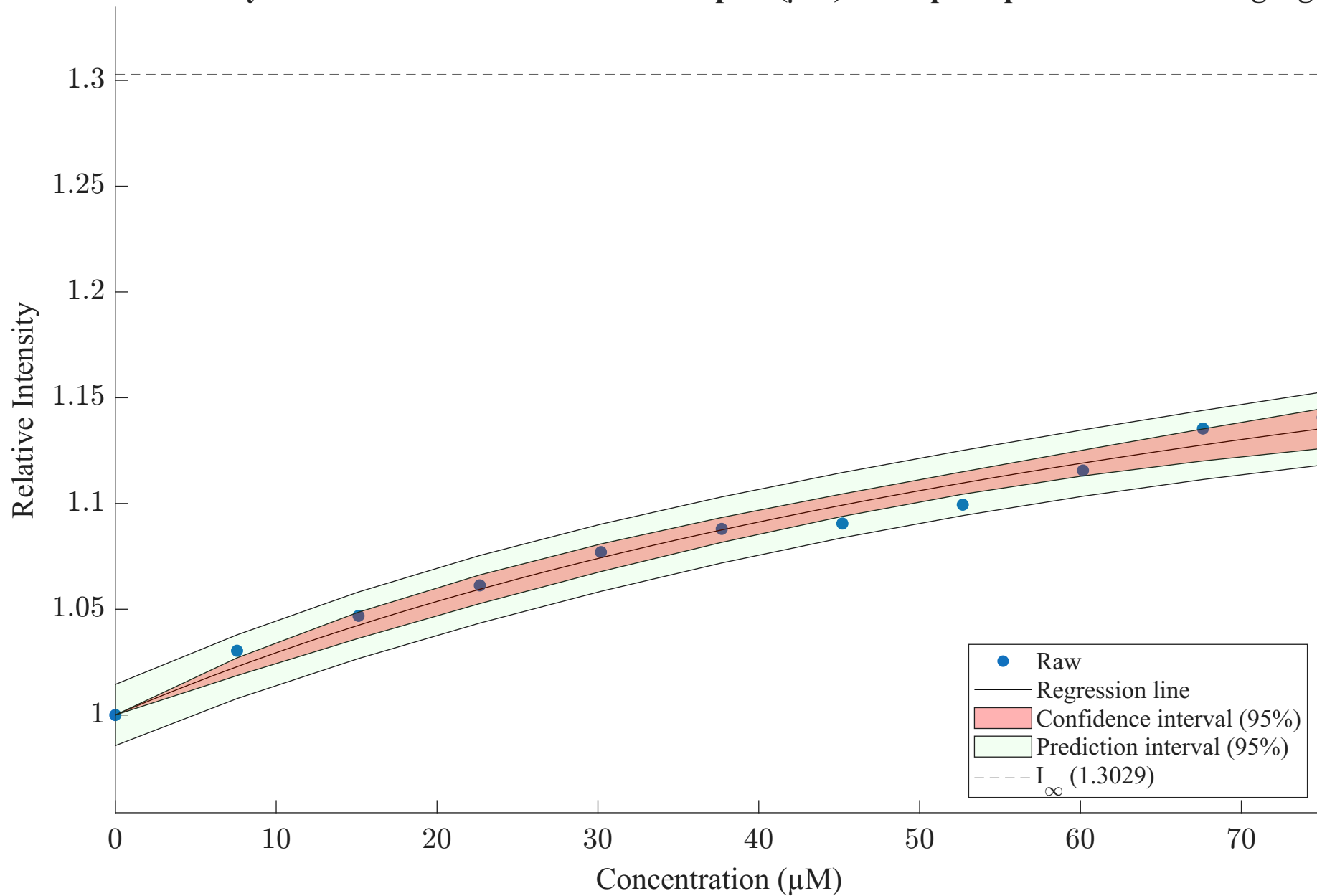
Relative intensity as a function of concentration of lipids ( \mu\text{M} ) for triple rep3 - Statistics fitting algorithm
